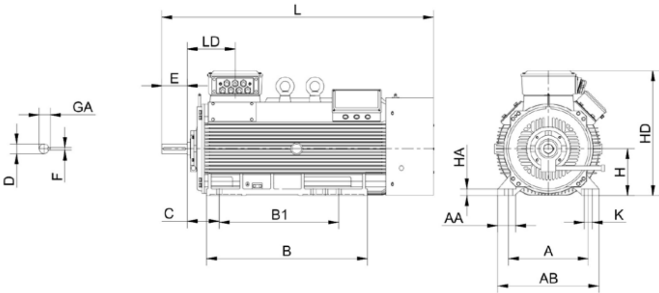
OMT1C IE3 FW DIMENSIONS
